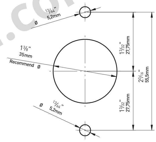
Fixing template
